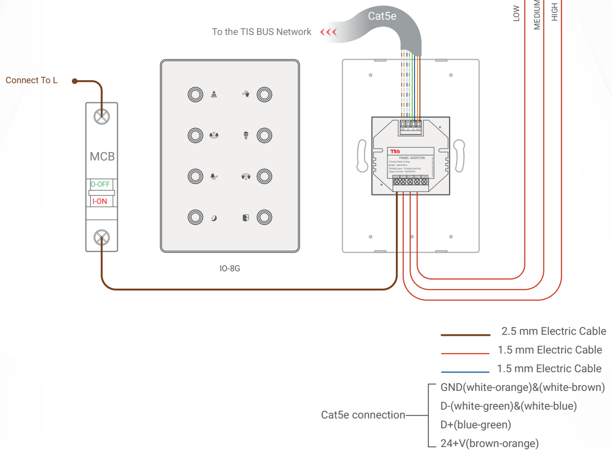
▲ Figure 2: IO 8G & ADD-3R-5A & High/Med/Low FCU Unit Connection Diagram
