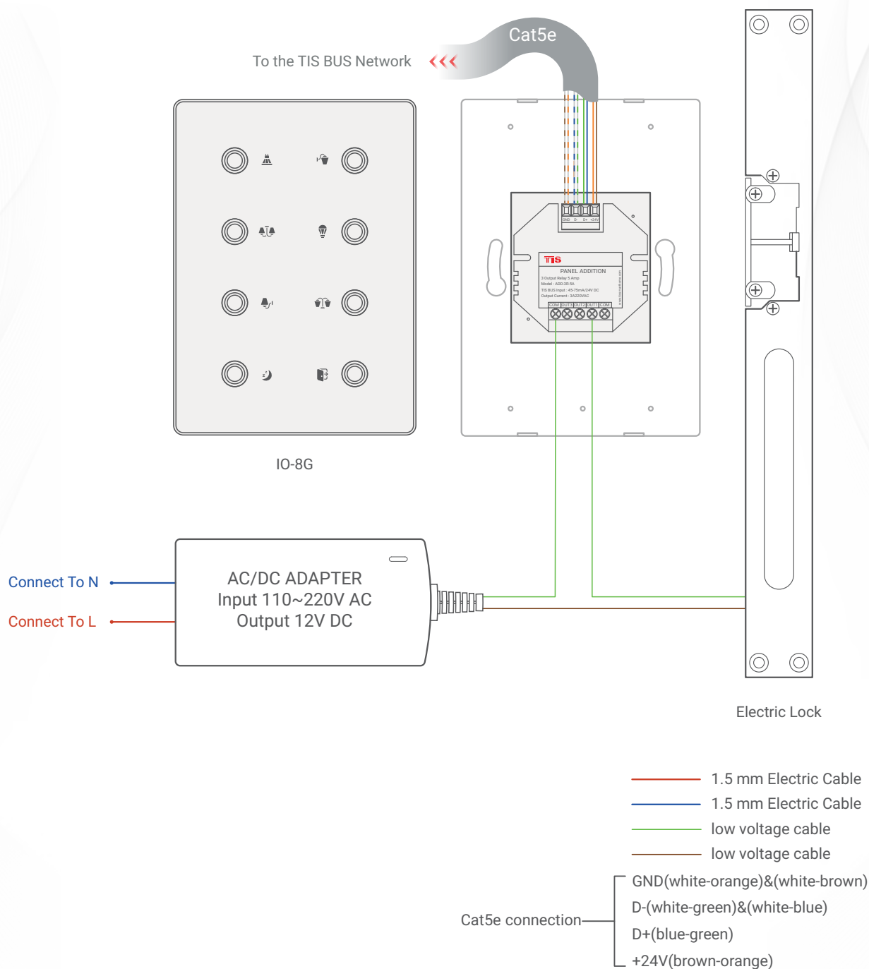
▲ Figure 5: IO 8G & ADD-3R-5A & Electric Lock Connection Diagram
