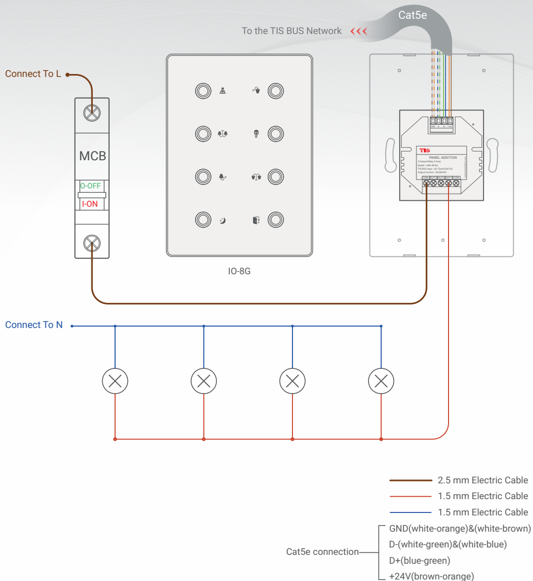
▲ Figure 1: IO 8G & ADD-3R-5A & Lights Connection Diagram
