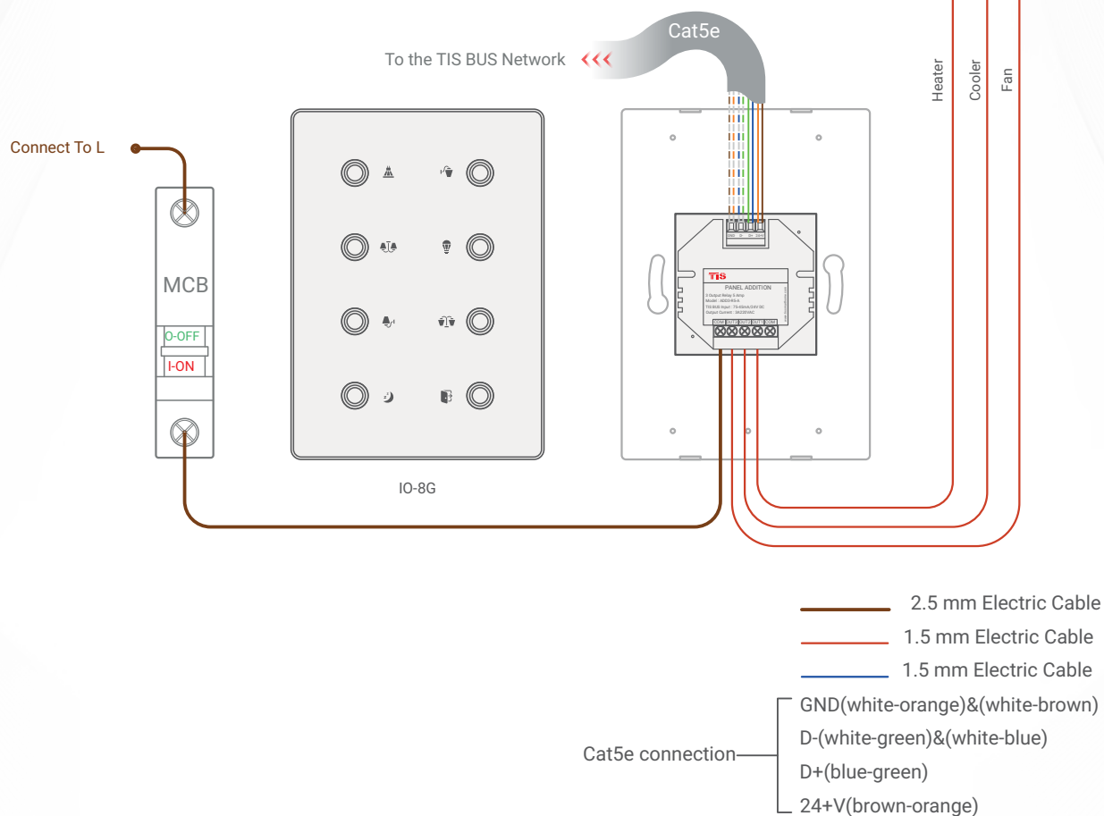
▲ Figure 3: IO 8G & ADD-3R-5A & Heater/Cooler/Fan FCU Unit Connection Diagram
