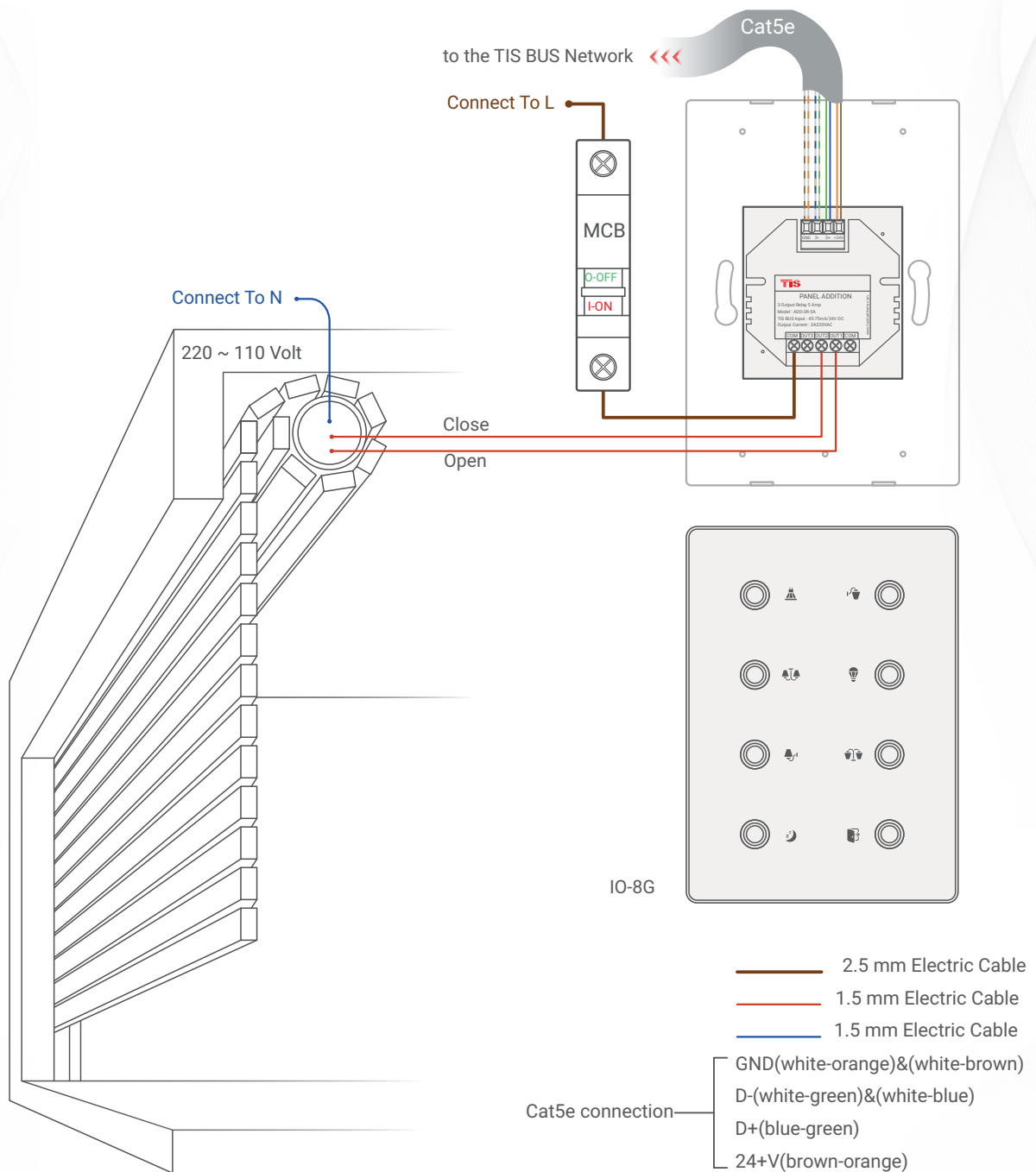
▲ Figure 4: IO 8G & ADD-3R-5A & Motors Connection Diagram
