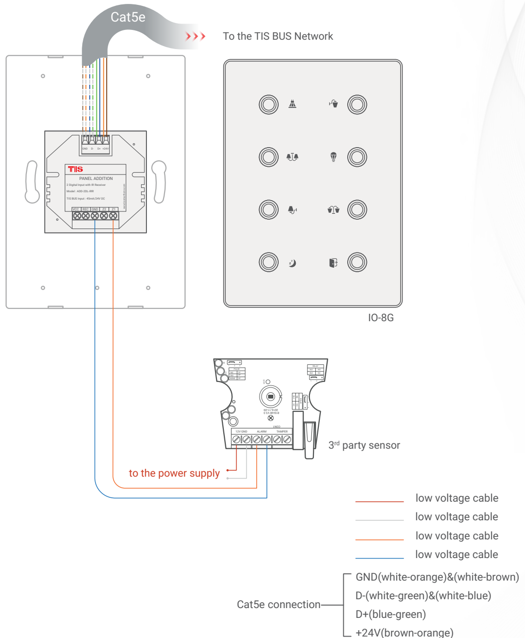
▲ Figure 10: IO 8G & ADD-2DL-IRR & 3 rd Party Sensor Connection Diagram
