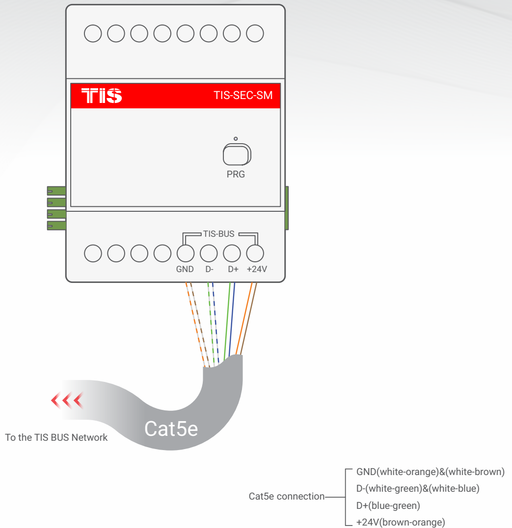
▲ Figure 1: Module's Bus Connection Color Coding Diagram
