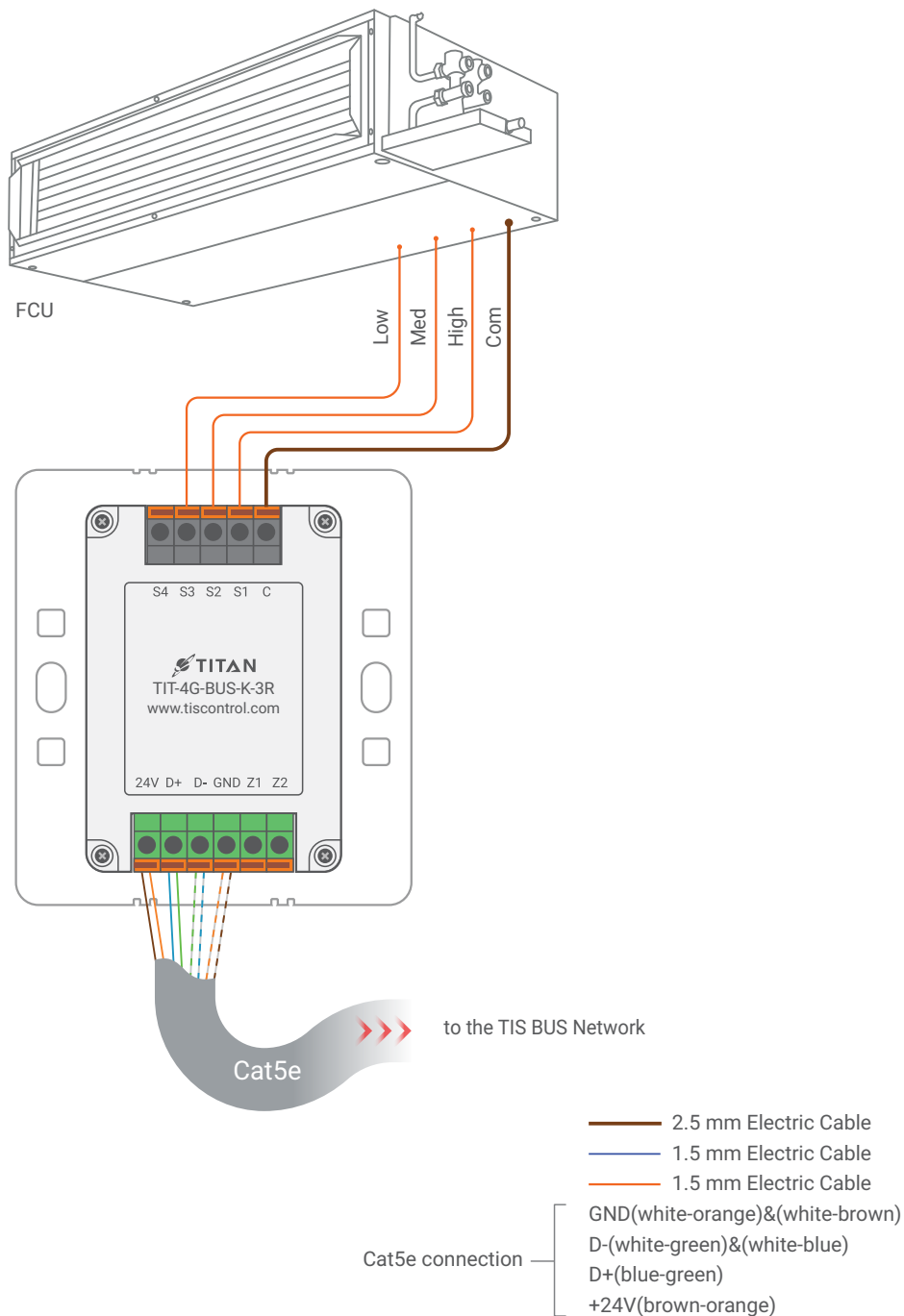
▲ Figure 2: TIT-4G-BUS-K-3R & FCU Connection Diagram
