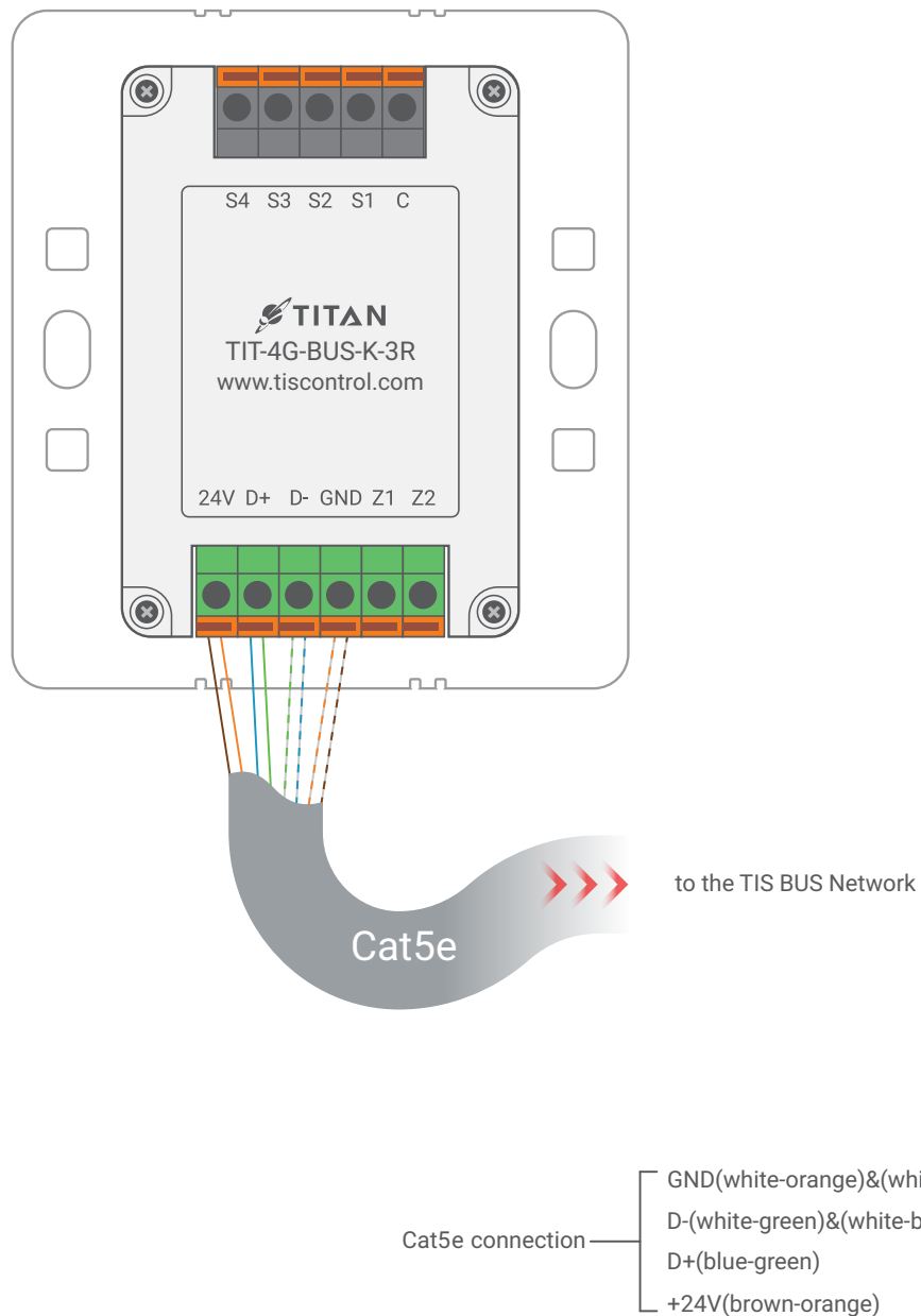
▲ Figure 7: TIT-4G-BUS-K-3R Module's Bus Connection Color Coding
