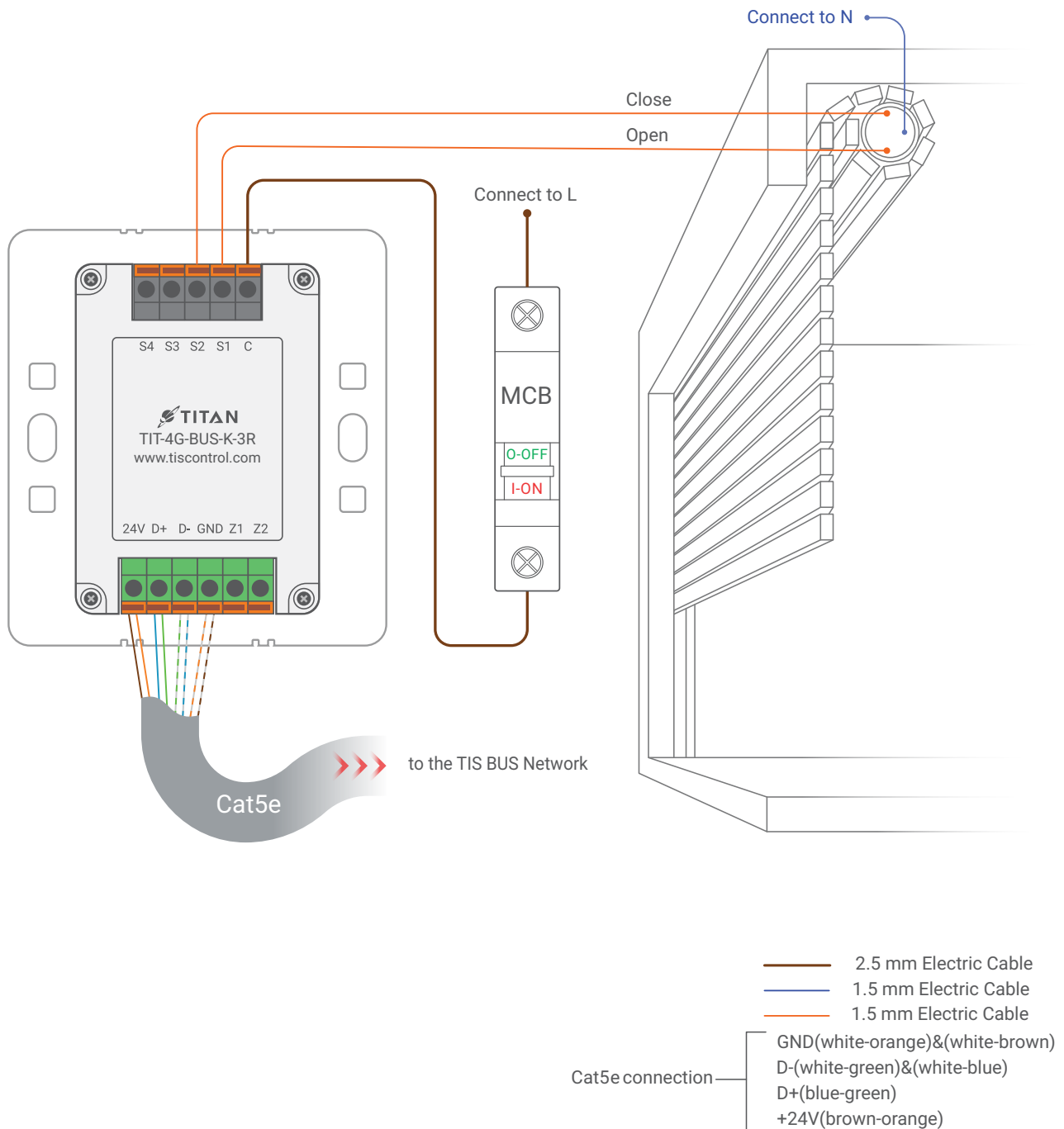
▲ Figure 4: TIT-4G-BUS-K-3R & Motors Connection Diagram
