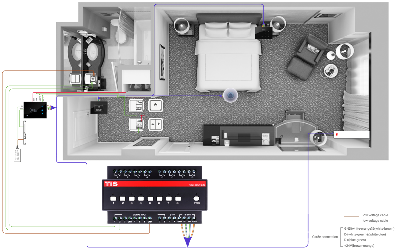
▲ Figure 1: Low Current Connection Diagram among Hotel Solutions
